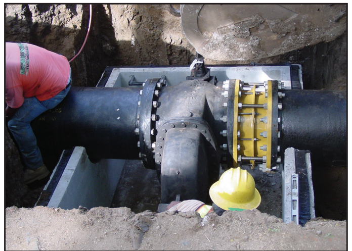
The Romac DJ400 combines a flanged spool piece with restraint tie-rods in one easy-to-use assembly.
