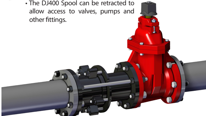
The Romac DJ400 combines a flanged spool piece with restraint tie-rods in one easy-to-use assembly.
