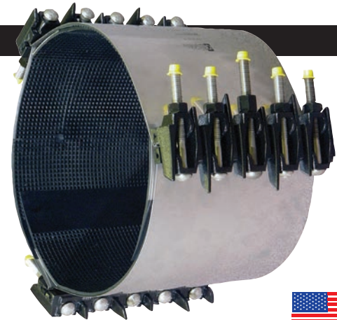
CL3-18.30 x 12" REPAIR CLAMP
