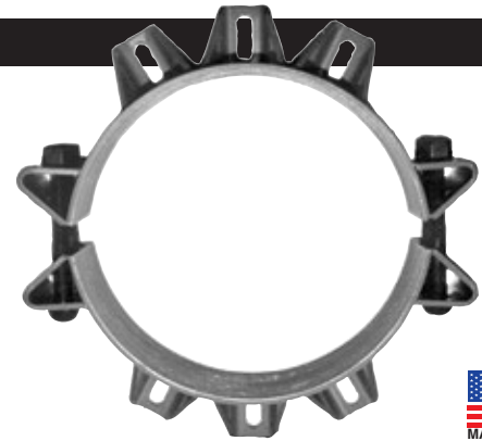
470 PIPE RESTRAINER
